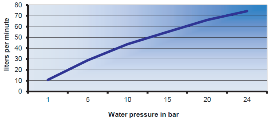
Water flow (INOX)
